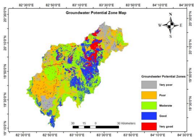
Figure 2. Groundwater Potential Zone Map
